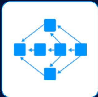
DAG Structure
